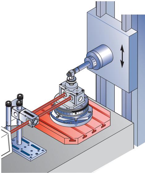
55290A Optical setup on horizontal machining center with vertical table (right) and with horizontal table
